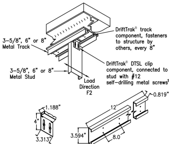
Figure 10 – DriftTrak® DTSL
