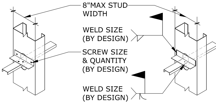
OPTION 1: SCREWED ATTACHMENT OF LATERAL BRACING
