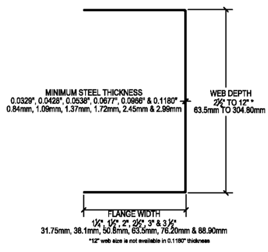
STRUCTURAL TRACK
