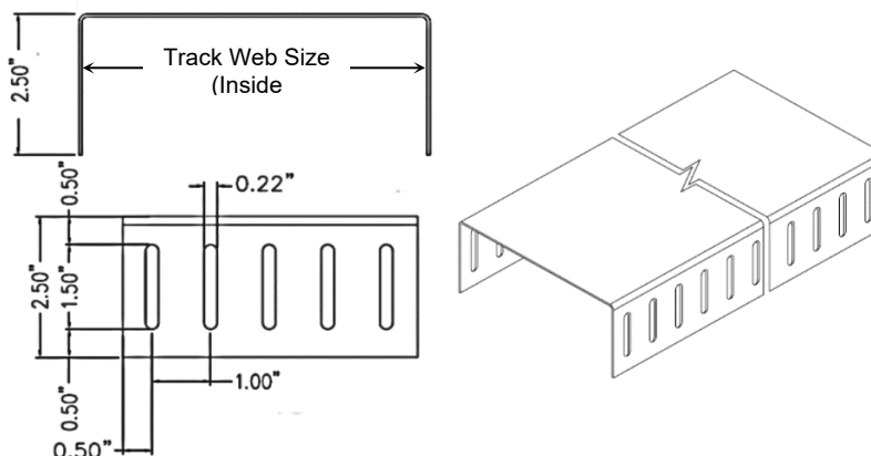
TRACK (Slotted Flange) xxxCST250 or xxxSLT250
